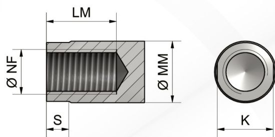
INTERIOR THREAD (code2)
