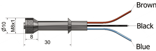
Straight plug - 3 m of cable
