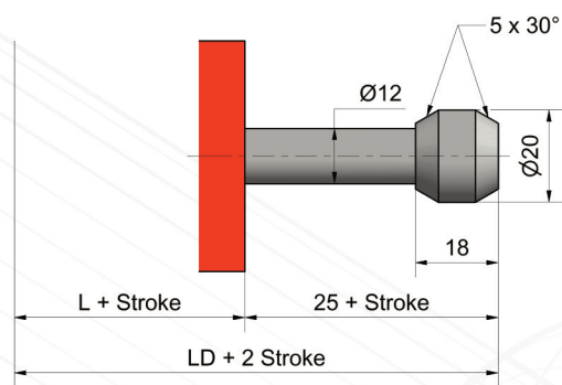
INFORMATION ROD (codeD)
